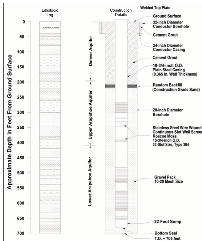
Lithologic Log and Well Construction Details
